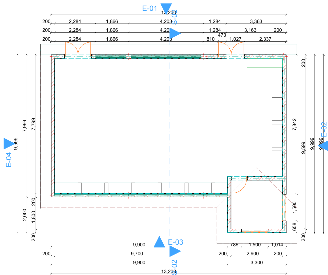
FLOOR LAYOUT PLAN
