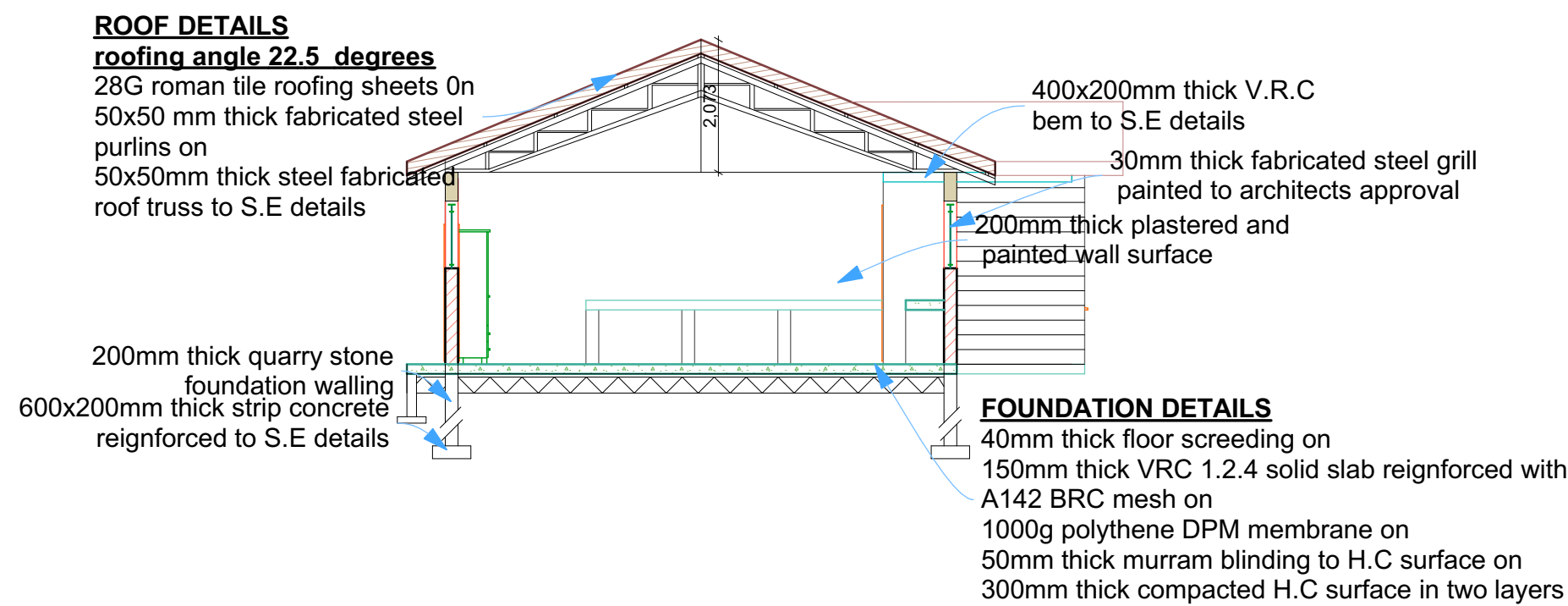
SECTION 02
