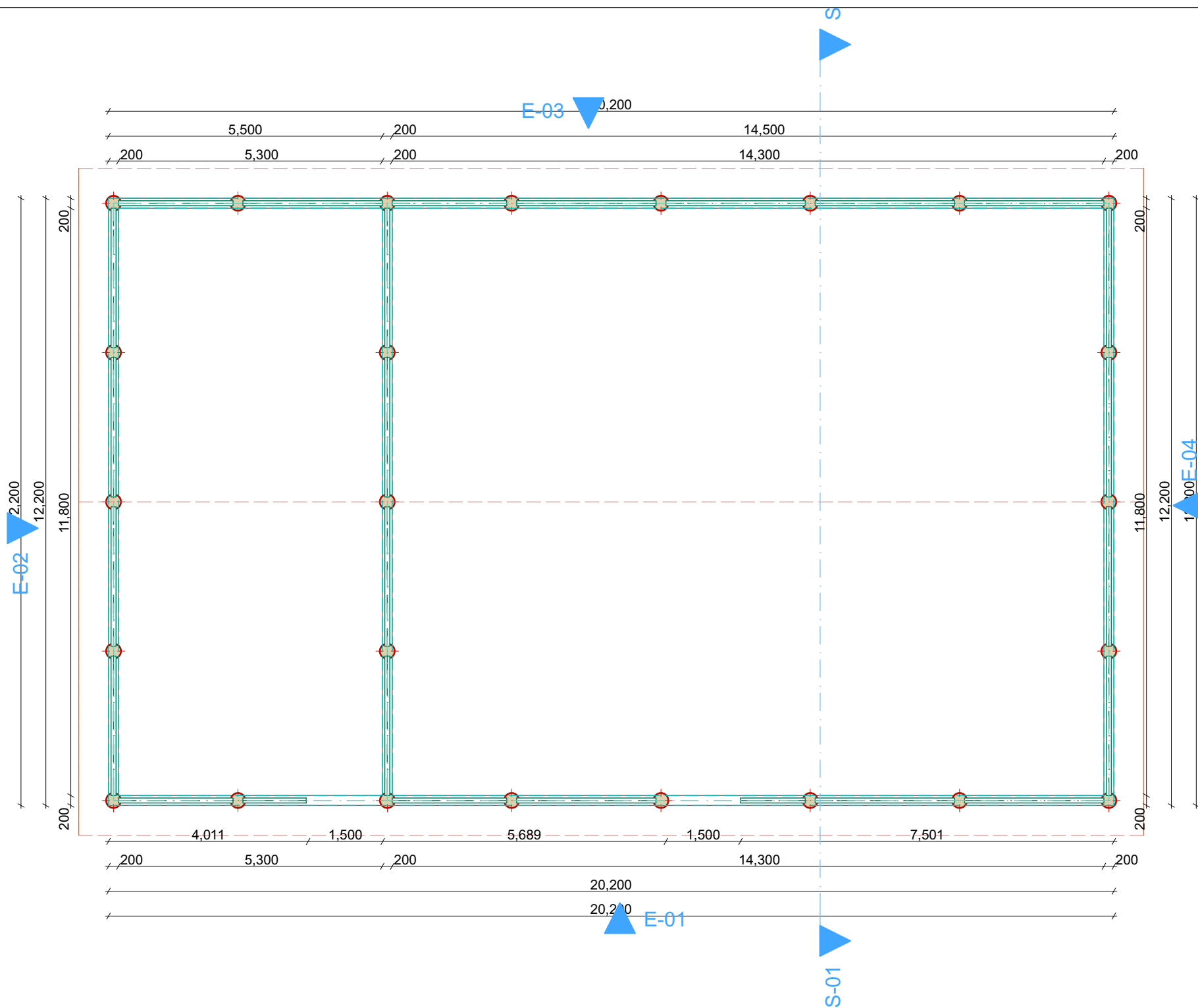
FLOOR PLAN LAYOUT
